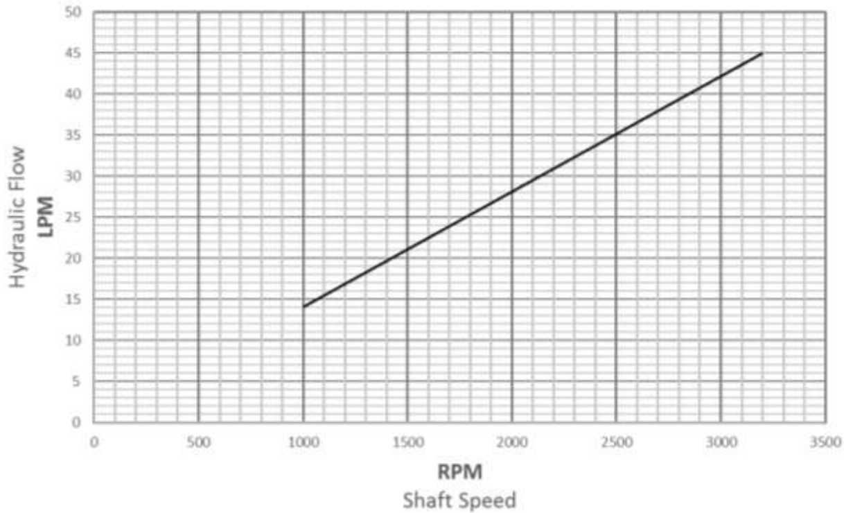
GR29 Hydraulic Flow Vs Shaft Speed
